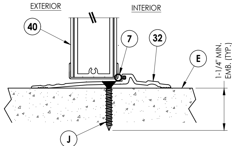
4 4 VERTICAL CROSS SECTION
