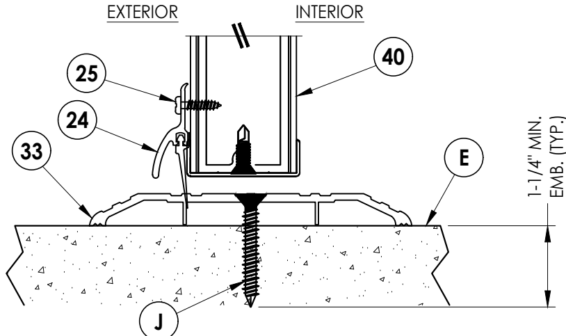
5 4 VERTICAL CROSS SECTION
